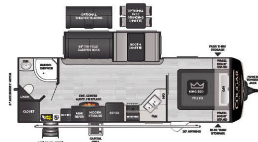
26RBSWE Rear bath w/ outside kitchen WEIGHT 6646 LENGTH 29' 11"
